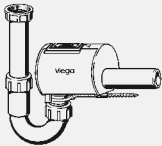
Sperrfix Backflow trap type 5
