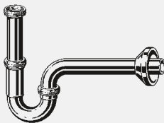
Pipe odour trap Plus siphon - brass Components adjusting pipe 120 mm, outlet elbow 220 mm quality controlled in accordance with EN 274 Model 5611.5
