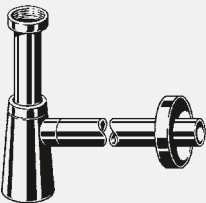
Eleganta 2 Bottle odour trap - chrome-plated brass Components adjusting pipe 200 mm, outlet pipe 310 mm, rosette Ø32xØ80xH15 mm Model 5788.5
