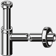
Eleganta 1 Bottle odour trap - chrome-plated brass Components adjusting pipe 200 mm, outlet pipe 310 mm, rosette Ø32xØ80xH15 mm Model 5788
