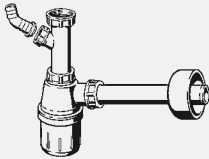
Bottle odour trap - plastic Components cup Ø 50 mm, waste water hose connection Model 5727
