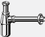
Bottle odour trap - chrome-plated brass Components cup Ø 60 mm, rosette, adjusting pipe 95 mm, outlet pipe 200 mm quality controlled in accordance with EN 274 Model 5763
