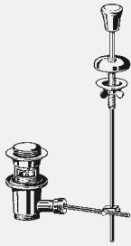
Drain - for WB with overflow Components draw button Model 5815
